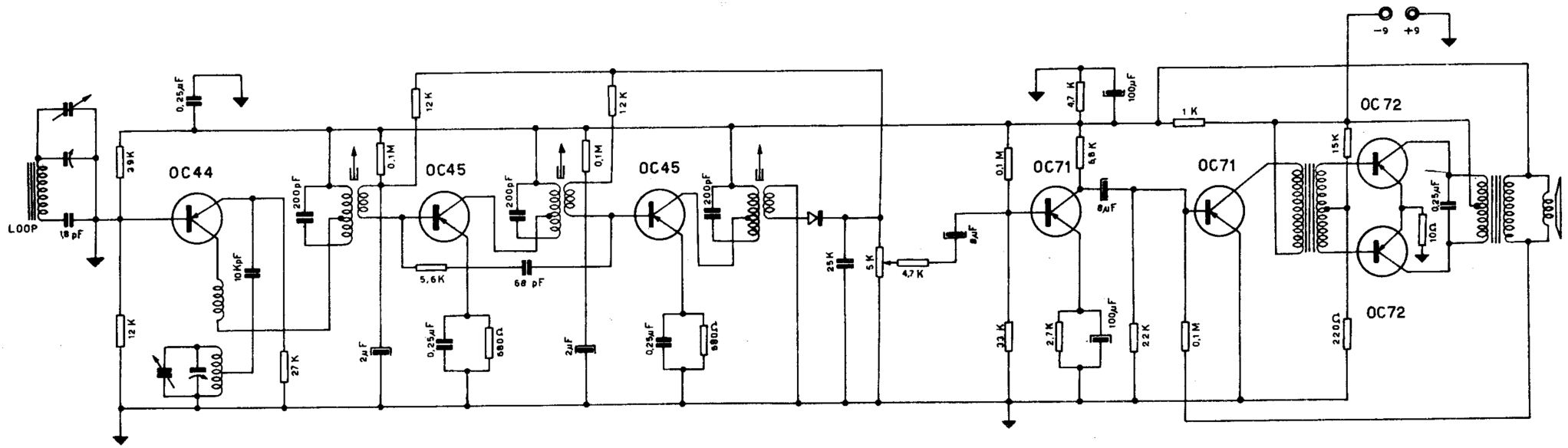
— RADIORICEVITORE A TRANSISTORS mod. R77 —
